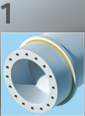
Ring seal repair and finishing Sikaflex®-521UV Sikaflex®-221
