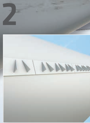
Re-Attachment of parts SikaForce®-7818 L7 Sikasil®AS-785
